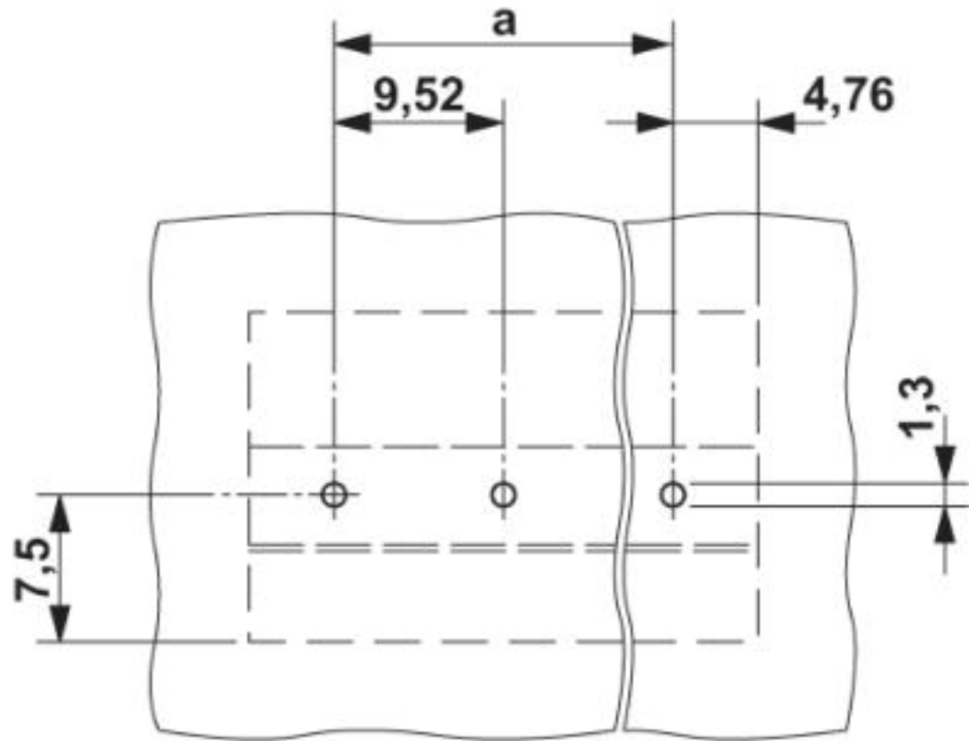
Drilling diagram
